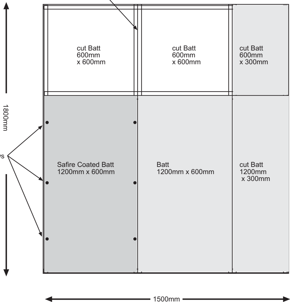
DETAIL SHOWING FRONT SIDE OF LARGE OPENING
