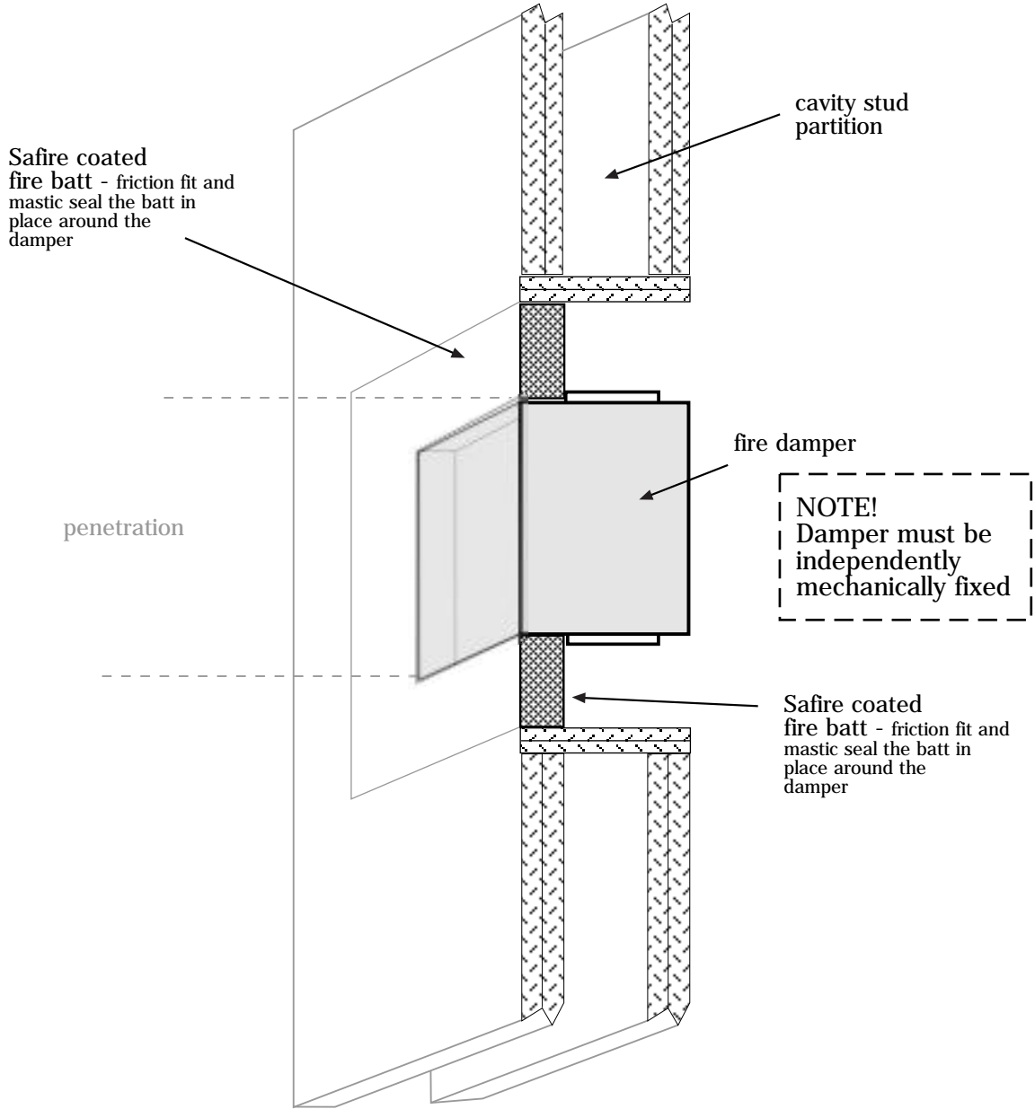
ISOMETRIC VIEW
